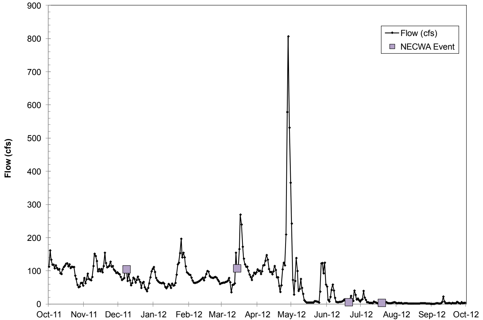
Figure 3-f. Flows during 2012 Coalition Monitoring: Pit River near Canby
