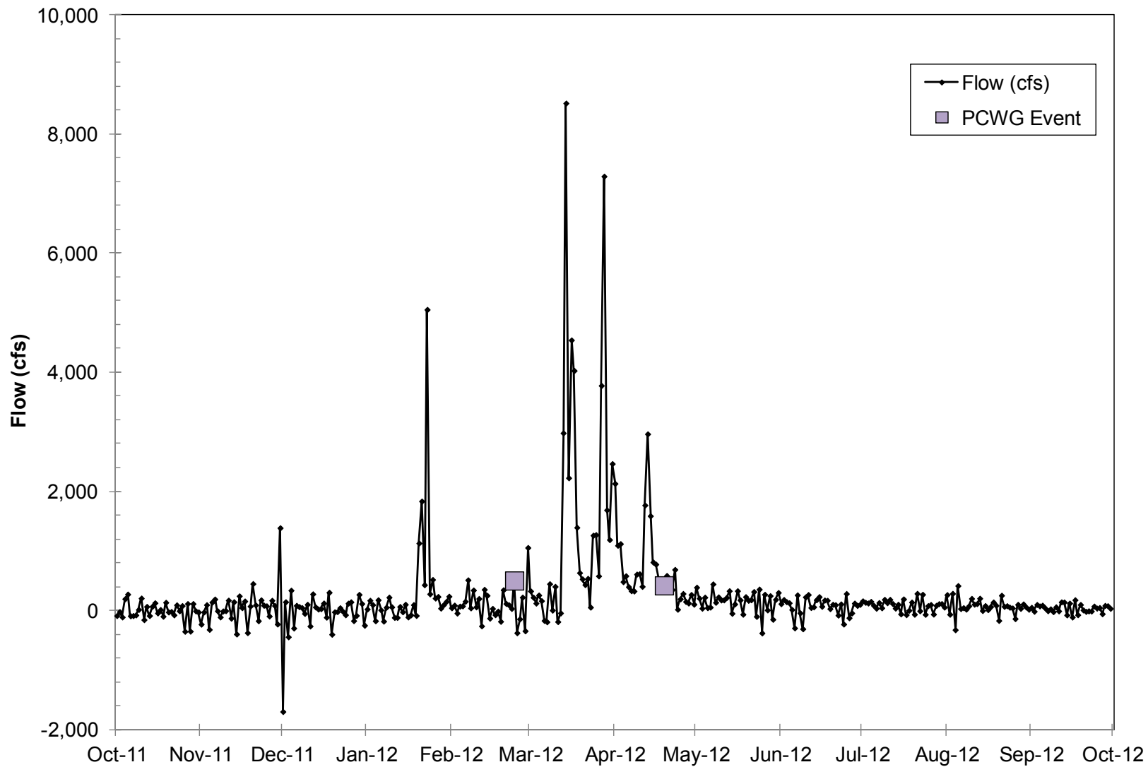
Figure 3-e. Flows during 2012 Coalition Monitoring: Lake Berryessa (Reservoir Inflow)
