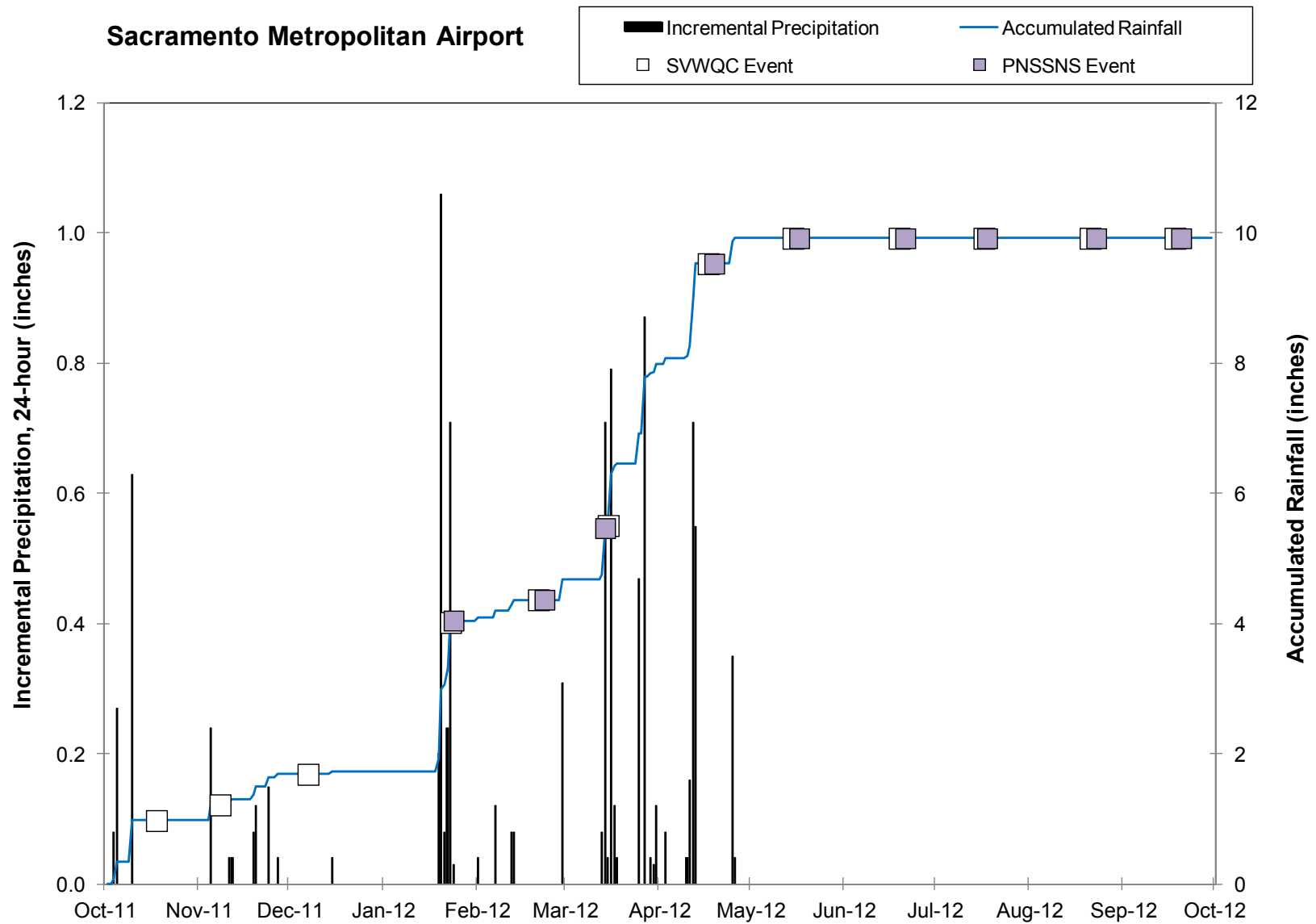
Figure 2-e. Precipitation during 2012 Coalition Monitoring: Lower Sacramento Valley
