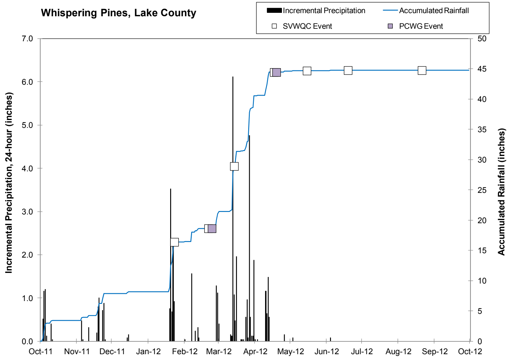
Figure 2-c. Precipitation during 2012 Coalition Monitoring: Lake County
