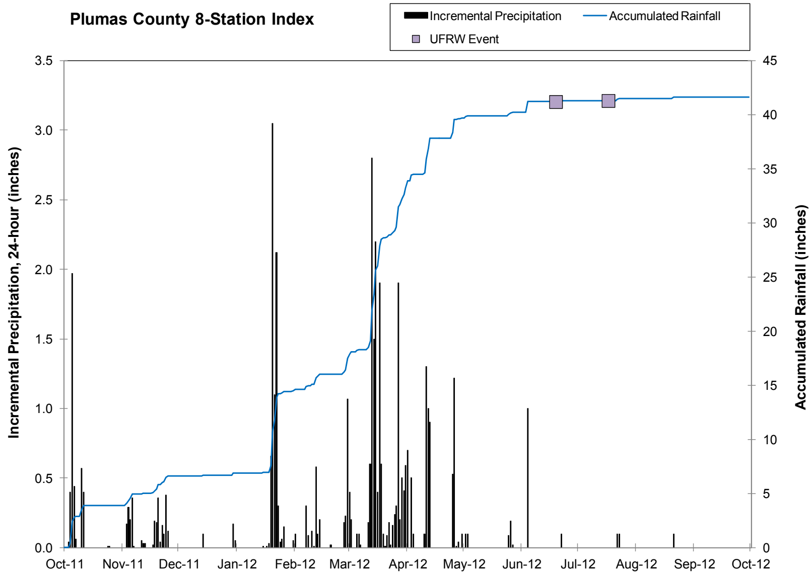
Figure 2-a. Precipitation during 2012 Coalition Monitoring: Plumas County
