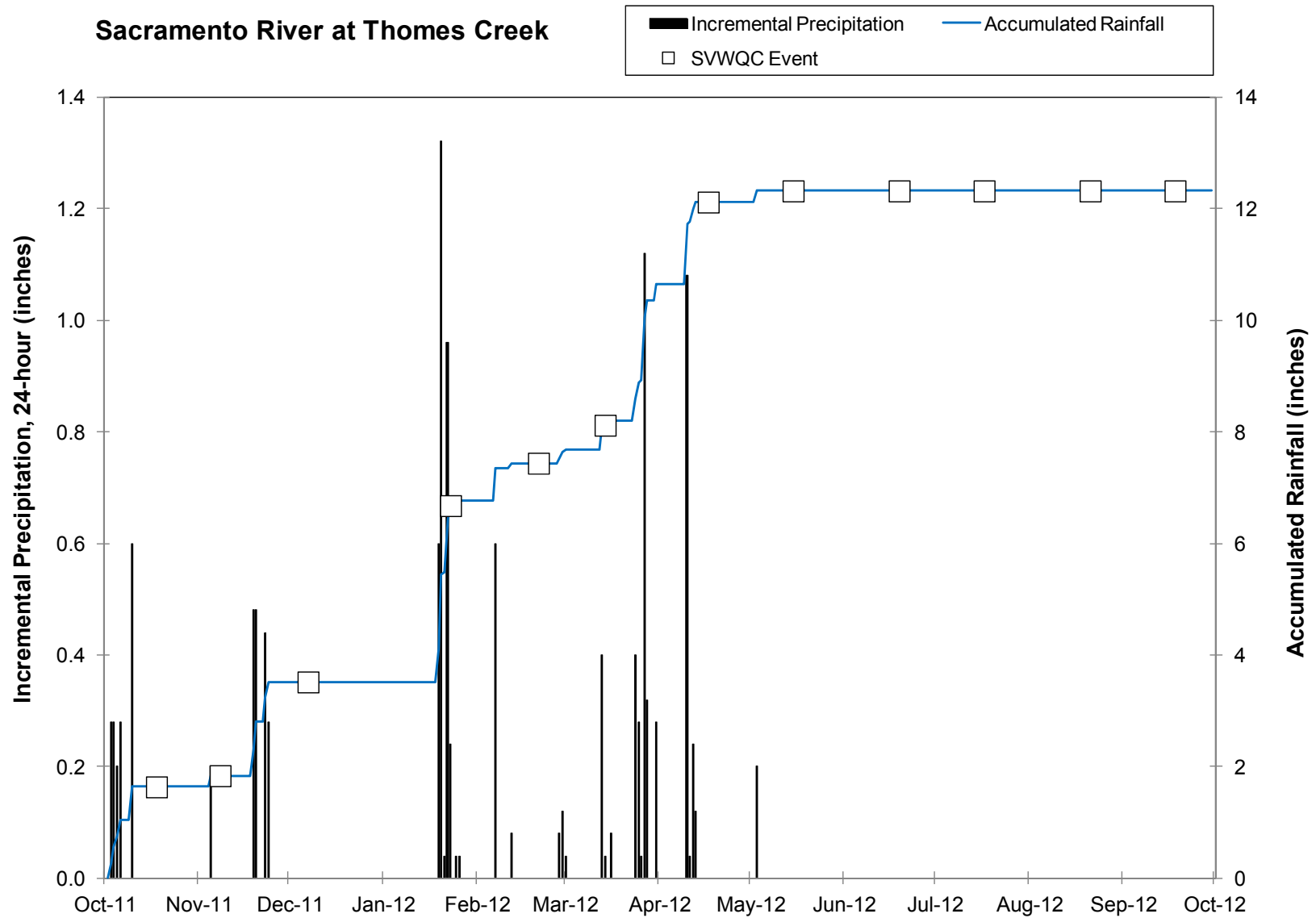
Figure 2-b. Precipitation during 2012 Coalition Monitoring: Upper Sacramento Valley
