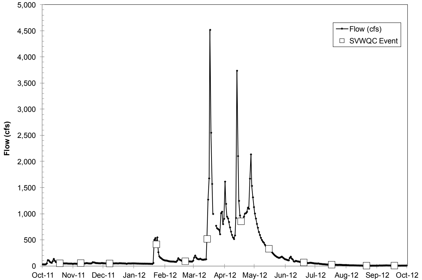
Figure 3-d. Flows during 2012 Coalition Monitoring: Lower Sacramento Valley
