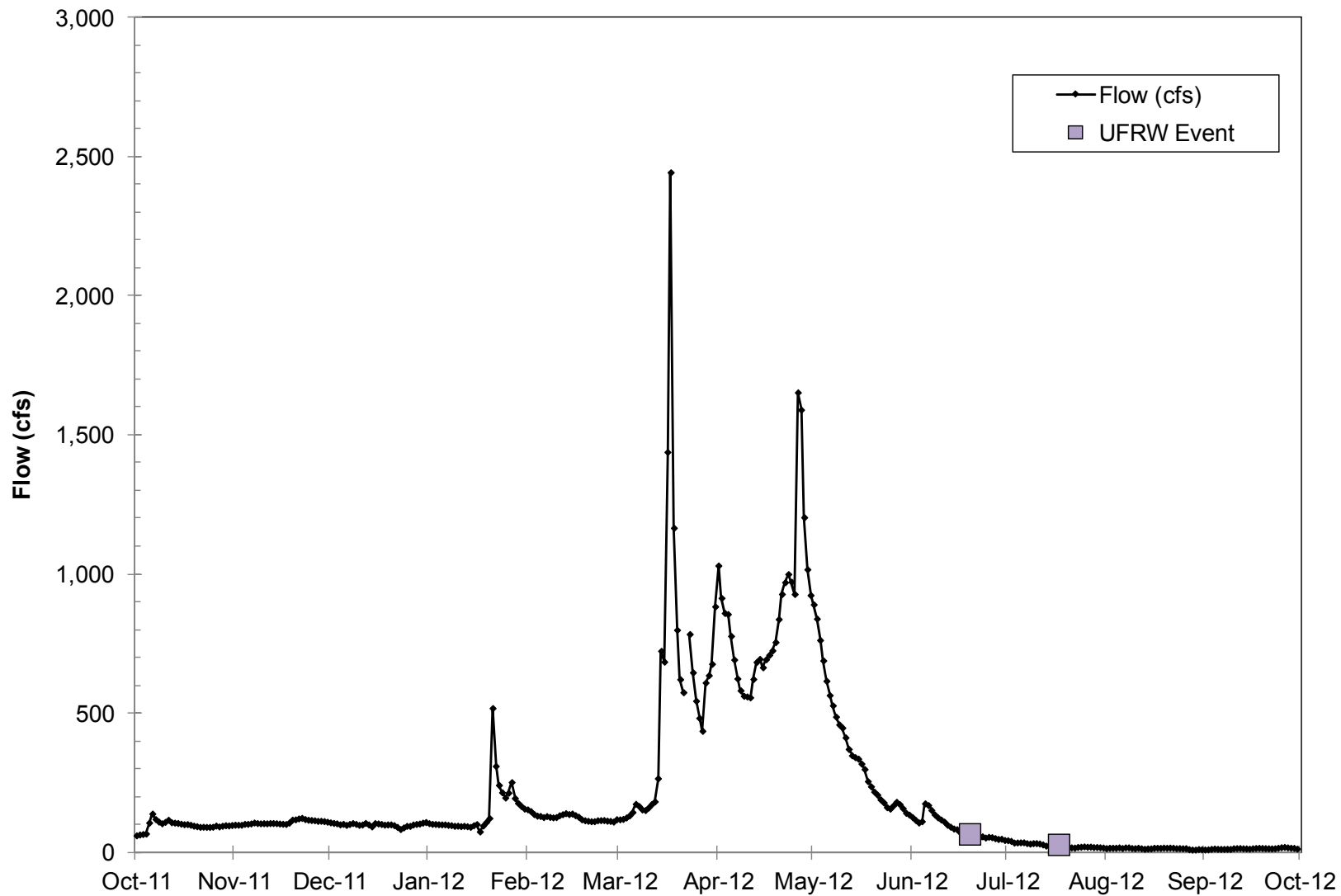
Figure 3-a. Flows during 2012 Coalition Monitoring: Plumas County
