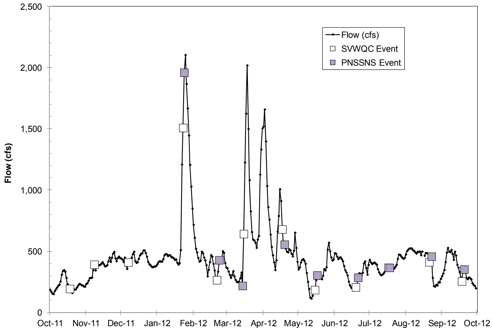
Figure 3-b. Flows during 2012 Coalition Monitoring: East Sacramento Valley
