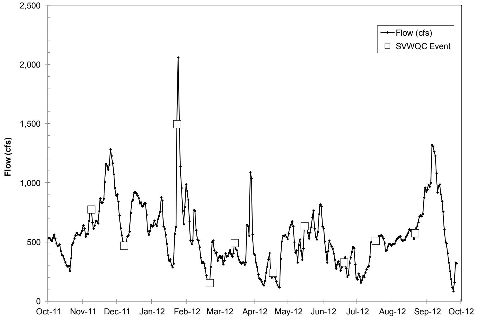
Figure 3-c. Flows during 2012 Coalition Monitoring: West Sacramento Valley
