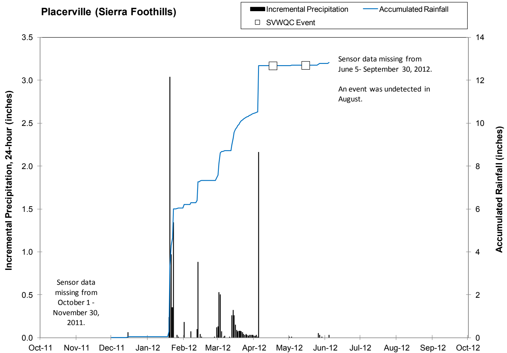
Figure 2-d. Precipitation during 2012 Coalition Monitoring: Sierra Foothills
