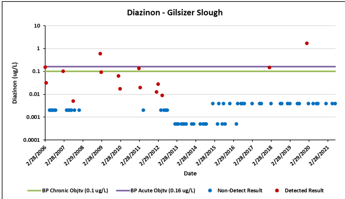
Figure 3. Diazinon Monitoring Results in Gilsizer Slough at George Washington Blvd: 2006 – 2021
